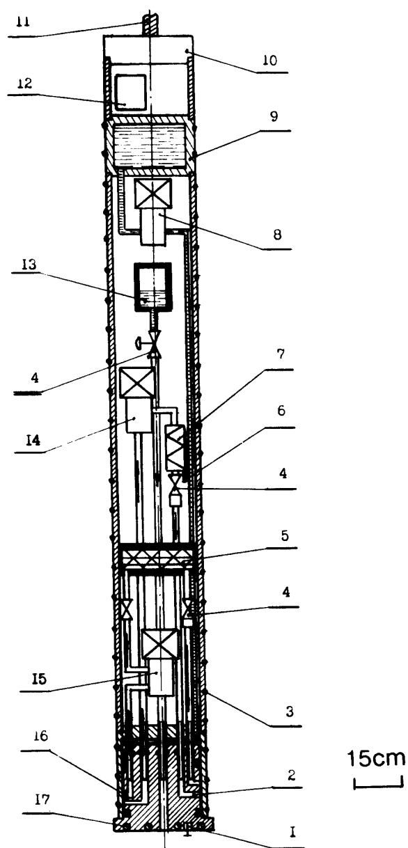
Fig. 5. The scheme of borehole sampling unit PSM-152.
