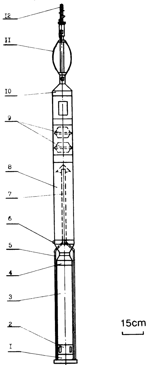
Fig. 2. The thermodrill TELGA-14M.
