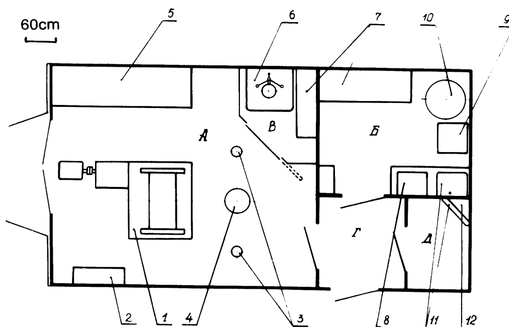
Fig. 1. Mobile microbiology drilling laboratory (MBU).
