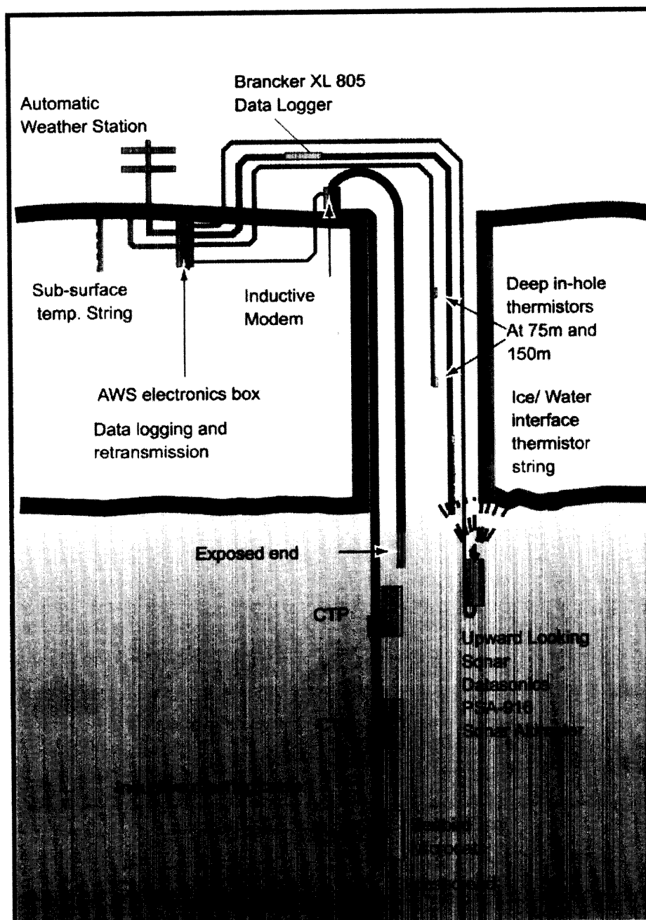
Fig. 5. Downhole instrumentation.
