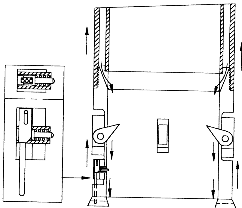
Fig. 5. Cutting head with core marking apparatus.
