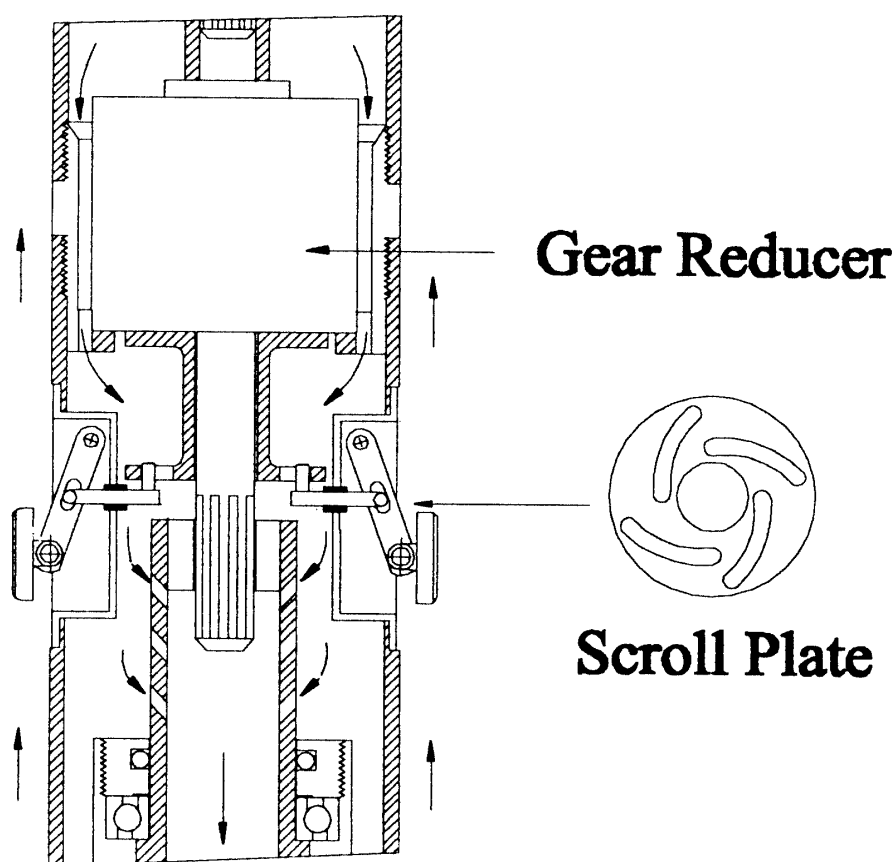
Fig. 3. Anti-torque mechanism.
