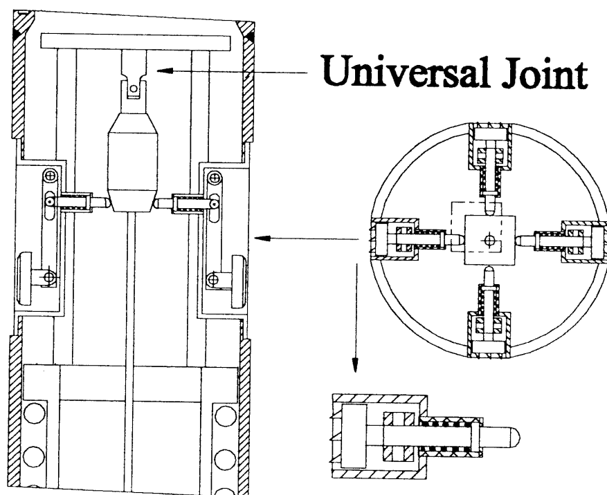
Fig. 2. Vertical stabilizer.
