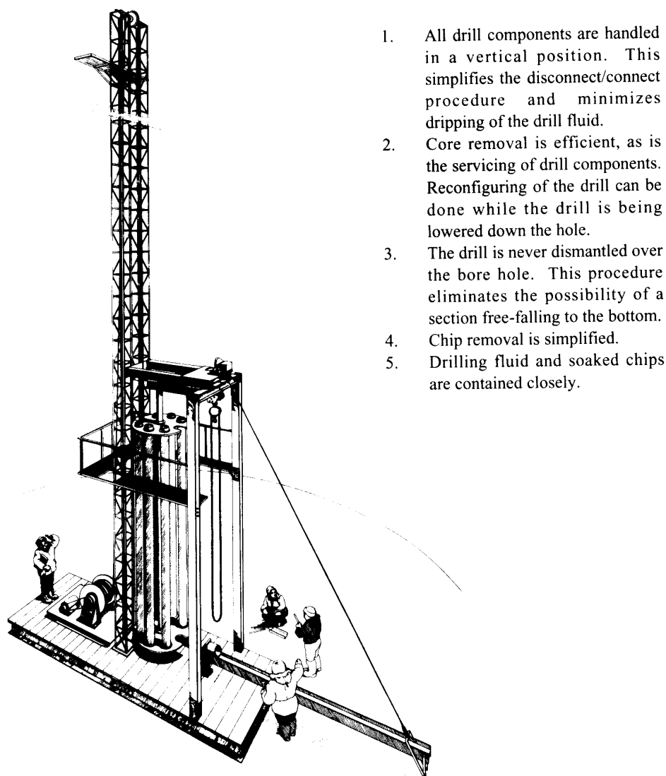
Fig. 11. Deep ice core drill handling system.
