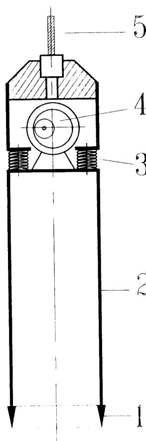
Fig. 14. Vibratory drill for drilling large-diameter boreholes in snow and firn.
