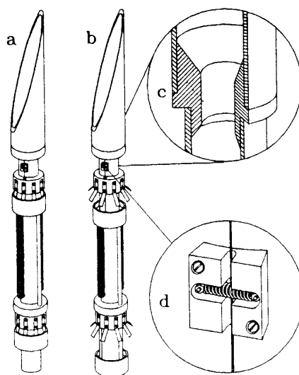
Whipstock : a - Lowering (initial) stage, b - working stage, c - neck, d - heating release mechanism.
