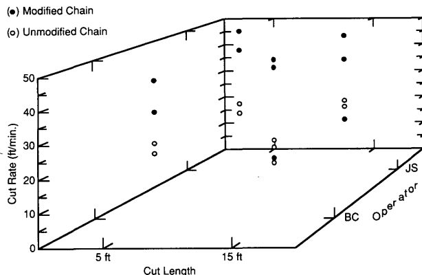
Figure 3. Ice cutting rate (in 7-in. ice) versus cut length and operator. The two outliers are the lower modified chain points at the 15-ft cut length with one for each operator.
