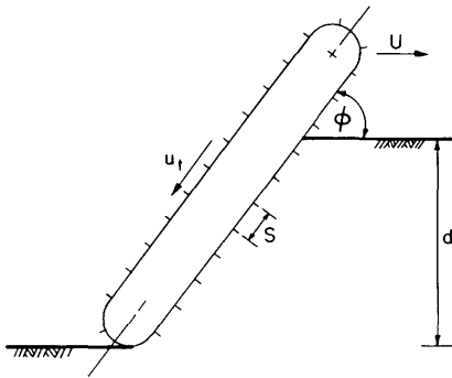
Figure 8. Chain saw blade and symbols used in the text (after Mellor 1976).
