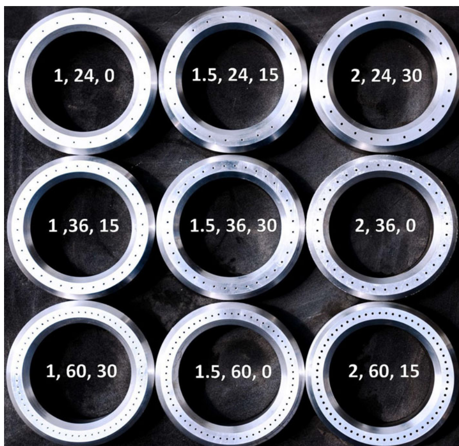
Fig. 3. Interchangeable drill heads; the numbers inside indicate diameter of the nozzles, the number of nozzles and angle from the vertical axis of the drill.
